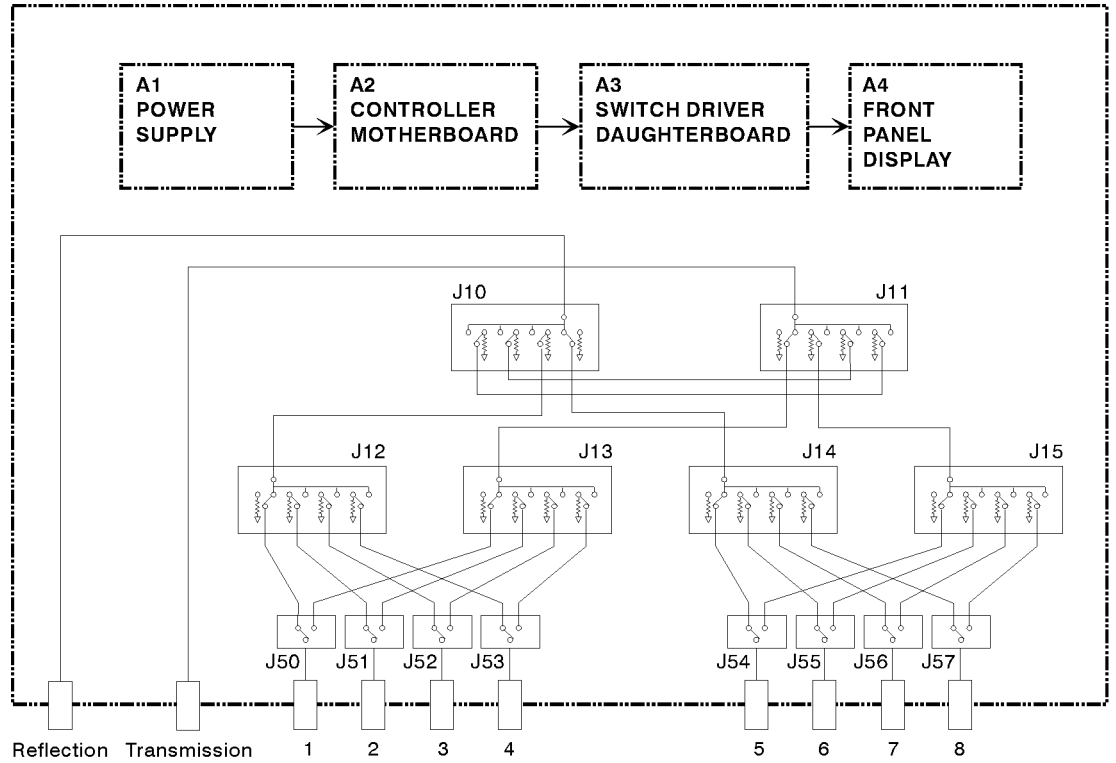
Figure 6-2. HP 87050A-H08 Block Diagram for Serial Numbers US 36130122 and above
