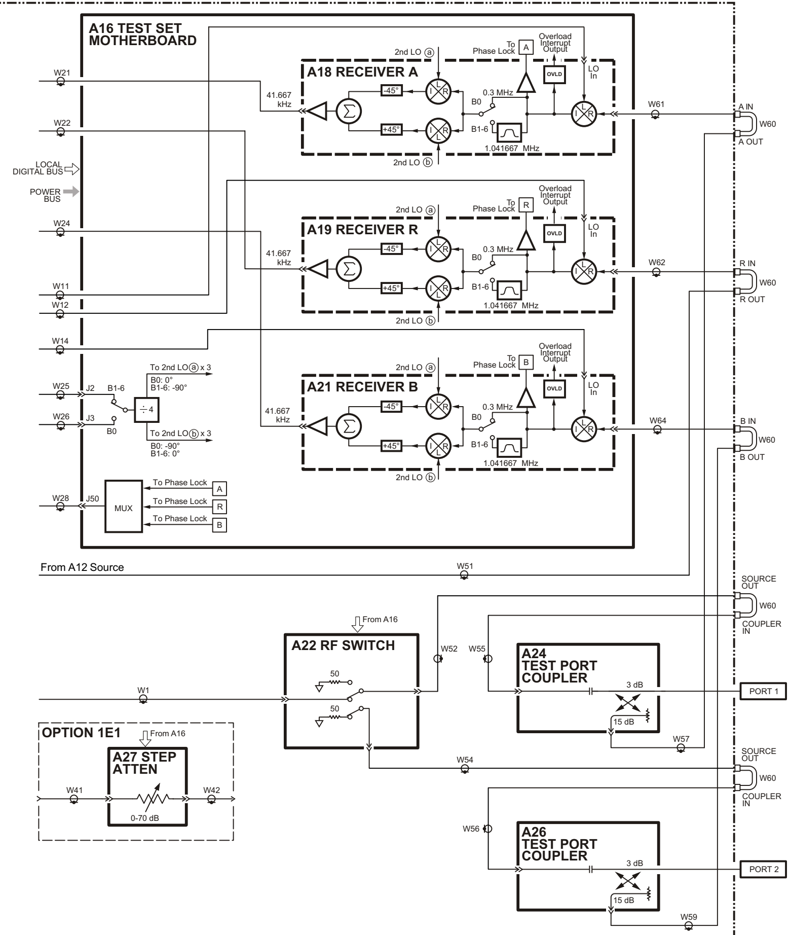
E8801A/02A/03A Option 014 Block Diagram Service Guide E8801-90001
